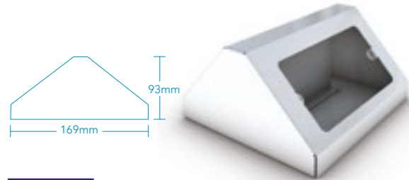
Part Code BS4 Twin. Back to back.
