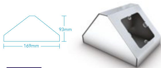
Part Code BS2 1 Gang. Back to back.
