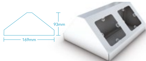
Part Code BS6 2x1 Gang Back to back.
